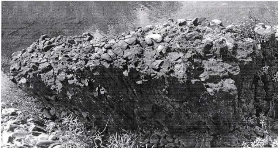
Autoclastic Conglomerate in Gud River channel
