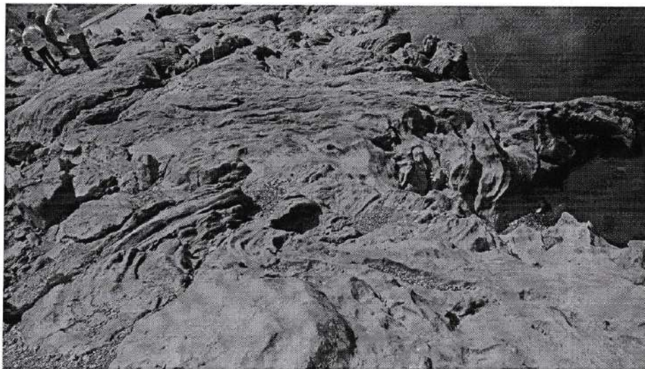
Folds in Metamorphic Rocks
