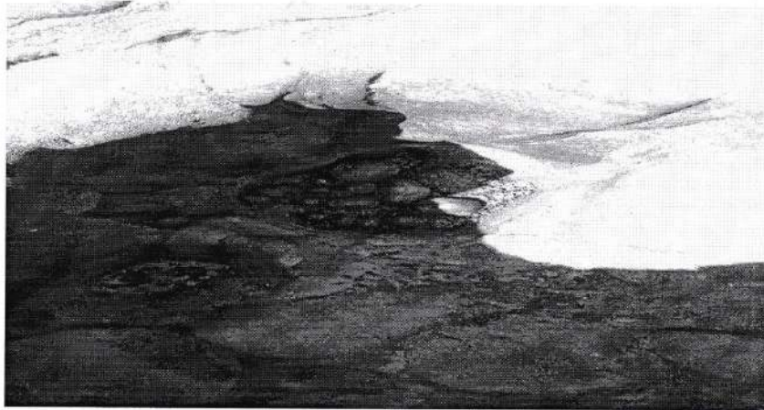
Potholes containing Pebbles at Gud River
