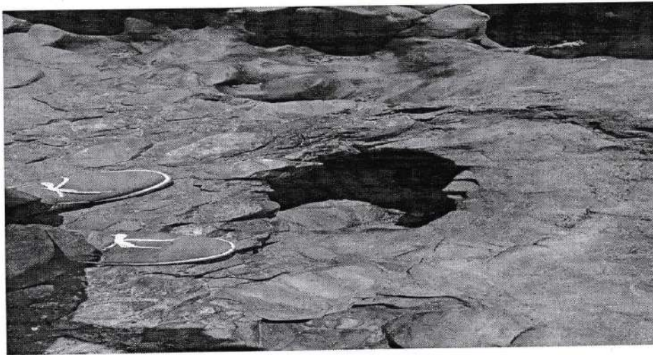
Potholes at Gud River
