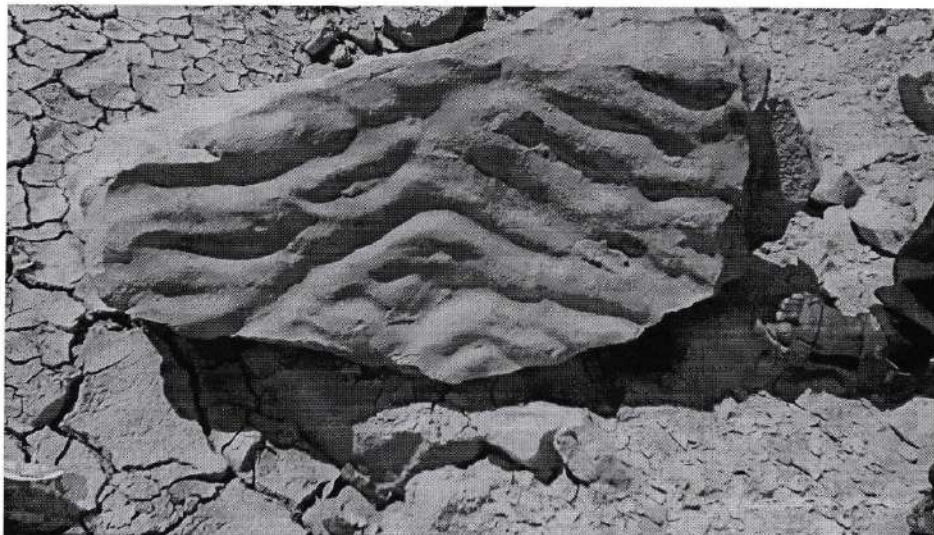
Ripple Marks in Sandstone near Fonda
